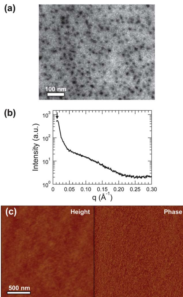
Fig. 5 Structure characterization of PF 9 - b -P4VP 231 : (a) TEM image and (b) SAXS curve for bulk samples. The TEM sample was stained with RuO 4 . (c) AFM images for a thin film ~65 nm in thickness.
