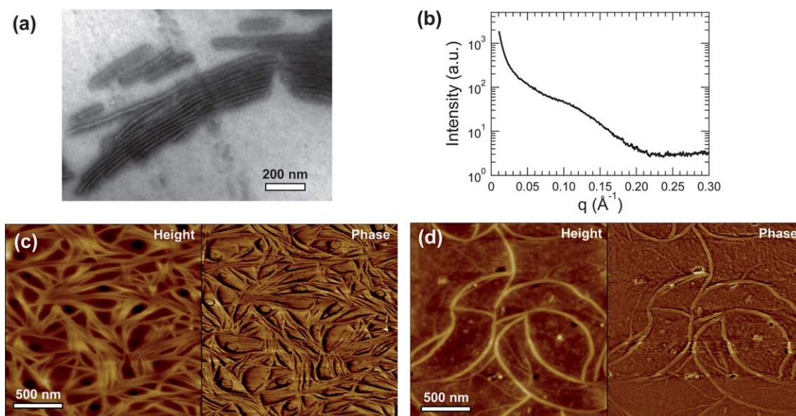
Fig. 3 Structure characterization of \text{PF}_9\text{-}b\text{-P4VP}_{22} : (a) TEM image and (b) SAXS curve for bulk samples. The TEM sample was stained with \text{RuO}_4 . AFM images for (c) a thicker film \sim 79 nm in thickness and (d) a very thin film (less than 18 nm).
