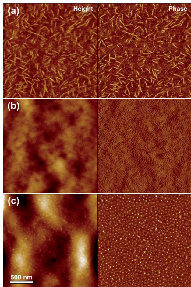
Fig. 7 AFM images for (a) a PF 9 - b -P4VP 22 (PDP) 1 thin film, thickness = 119 nm, (b) a PF 9 - b -P4VP 92 (PDP) 1 thin film, film thickness = 327 nm and (c) a PF 9 - b -P4VP 231 (PDP) 1 thin film, film thickness = 117 nm.
